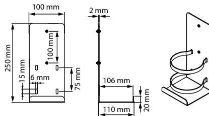
Pump Bracket
